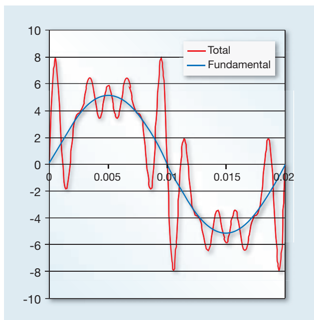
Figure 1: Voltage drop Waveform including harmonics
